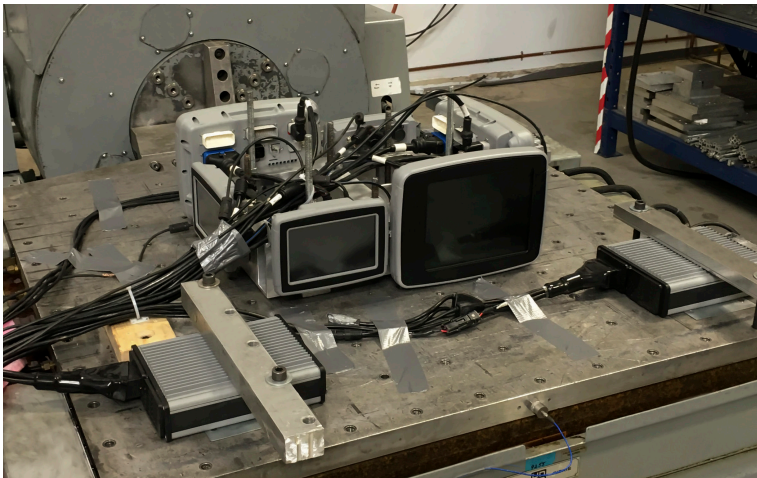
| Mechanical Loads Testing ISO 16750-3
